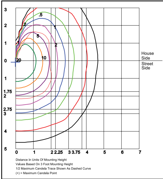
CAV7QC1X18U5K Grid in feet, Mounting Height = 3 ft.
