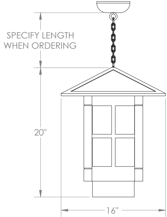
Chain Mount Chain ordered separately
