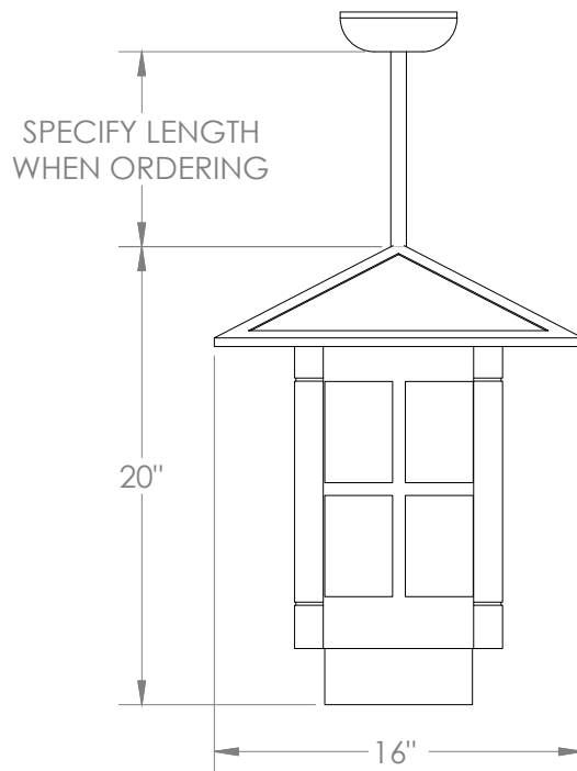
Stem Swivel Mount Stem ordered separately
