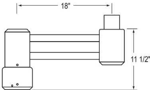
POST MOUNT PPMB14-SG-PM EPA: .7 WEIGHT: 65 lbs (max.)
